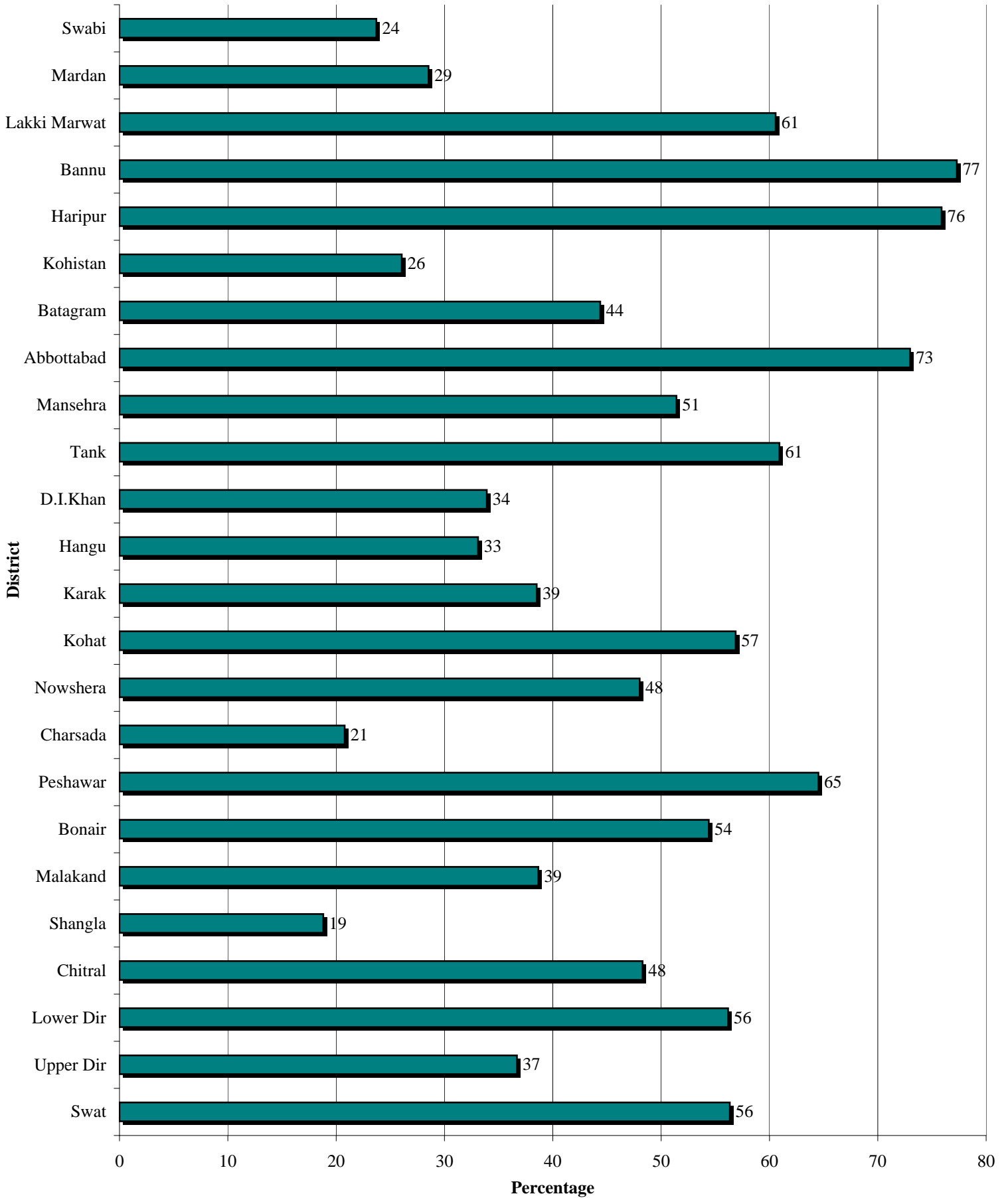
FIGURE 4.1 SOURCES OF DRINKING WATER AS PIPED - WATER N.W.F.P
